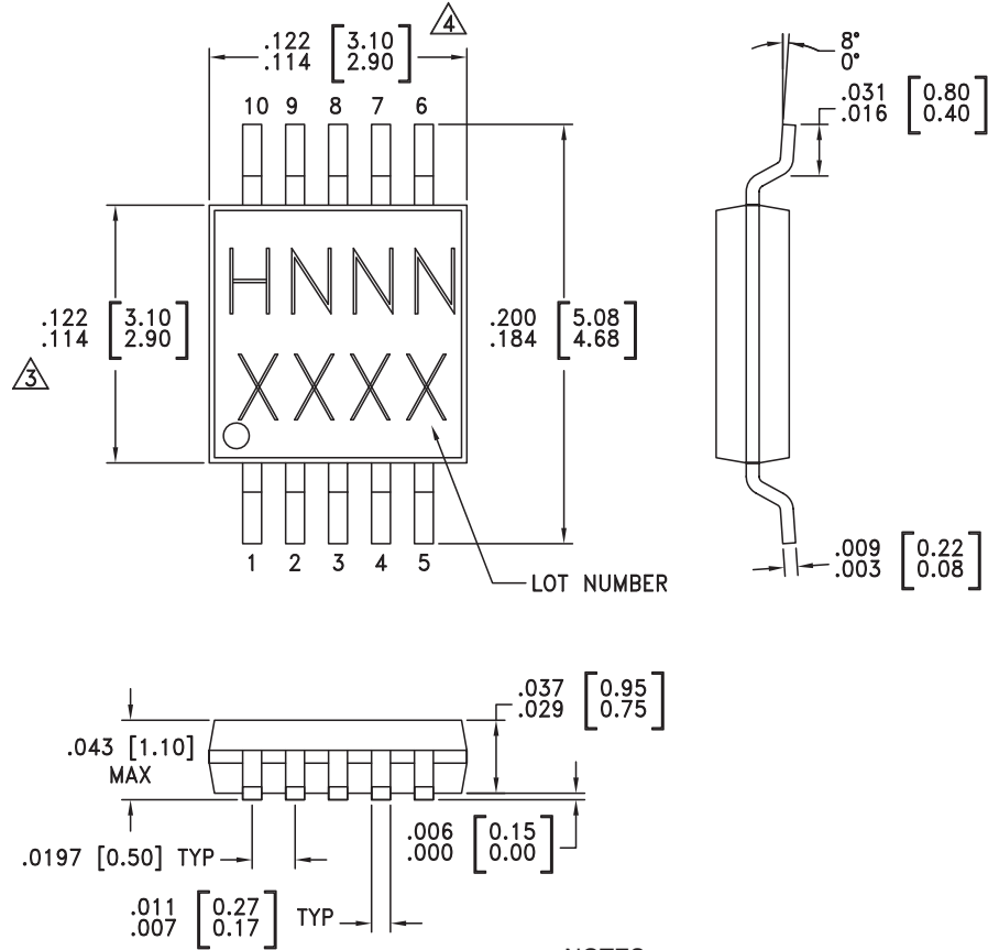
MS10 (E) Package Outline Drawing
